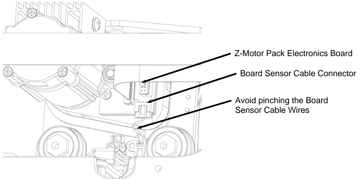
FIGURE 14: VIEW OF THE BACK OF THE Y-TRUCK
