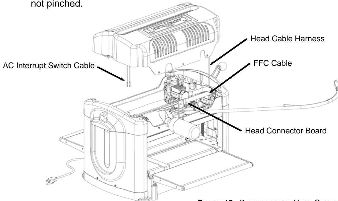
FIGURE 18: RESEATING THE HEAD COVER
