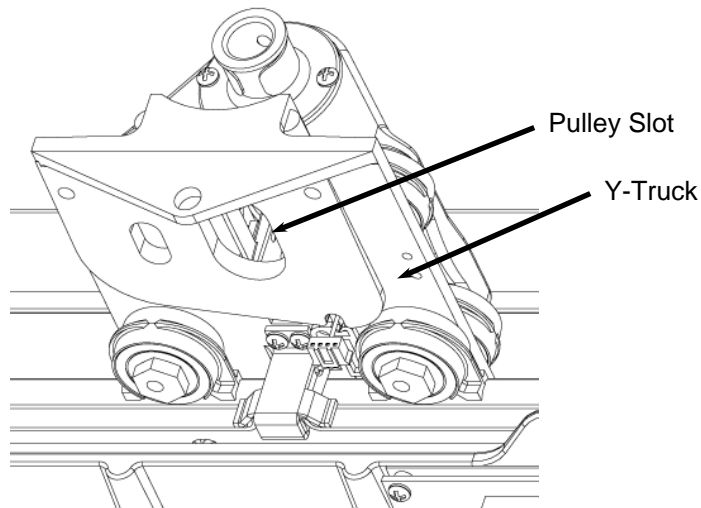
FIGURE 13: BACK OF THE Y-TRUCK
