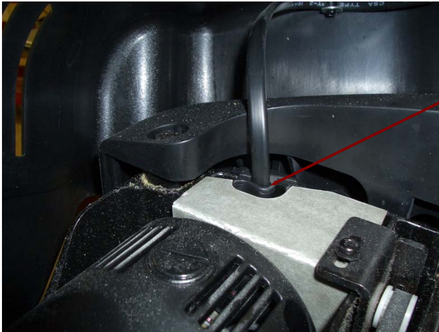
PICTURE 3: LOCATION OF AC INTERRUPT SWITCH CABLE WIRE RETAINER
