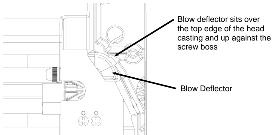
FIGURE 16: PLACEMENT OF THE BLOW DEFLECTOR - TOP
