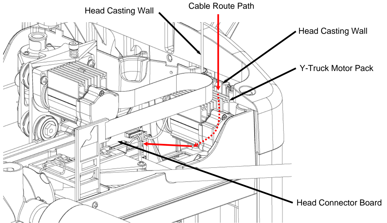
FIGURE 17: ROUTING THE HEAD CABLE HARNESS
