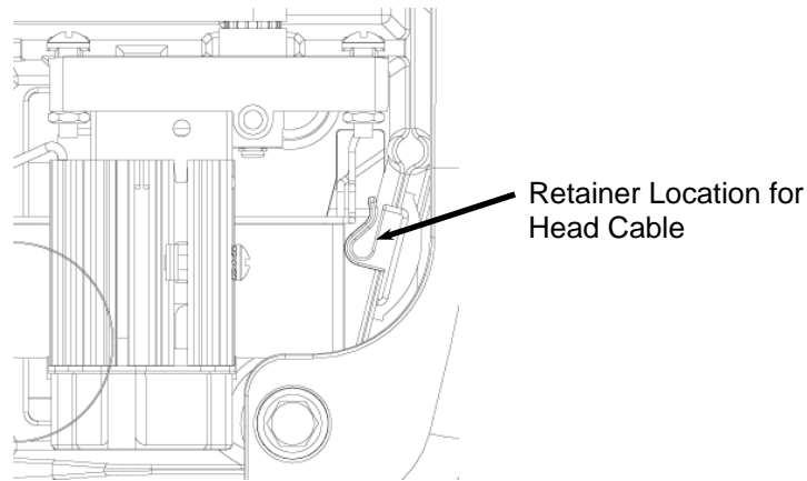
FIGURE 18: LOCATING THE HEAD CABLE HARNESS RETAINER
