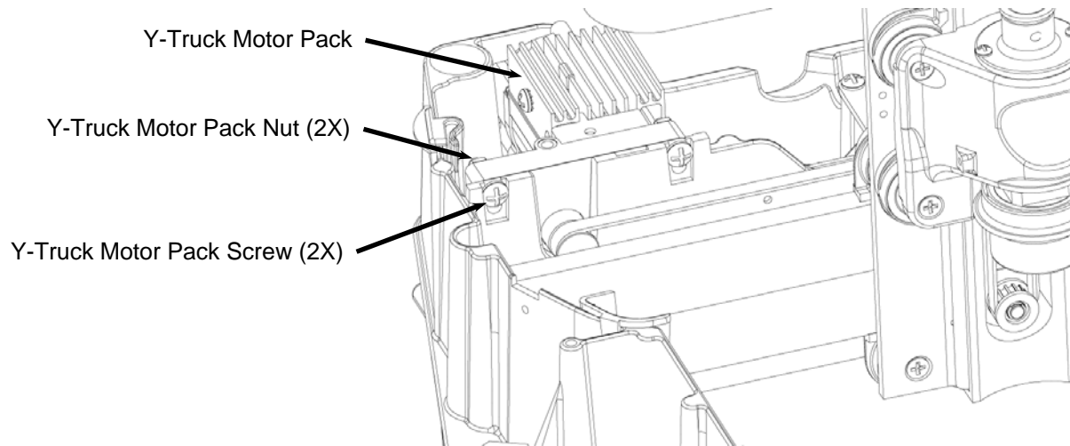
FIGURE 12: LOCATION OF Y-DRIVE MOTOR PACK SCREWS
