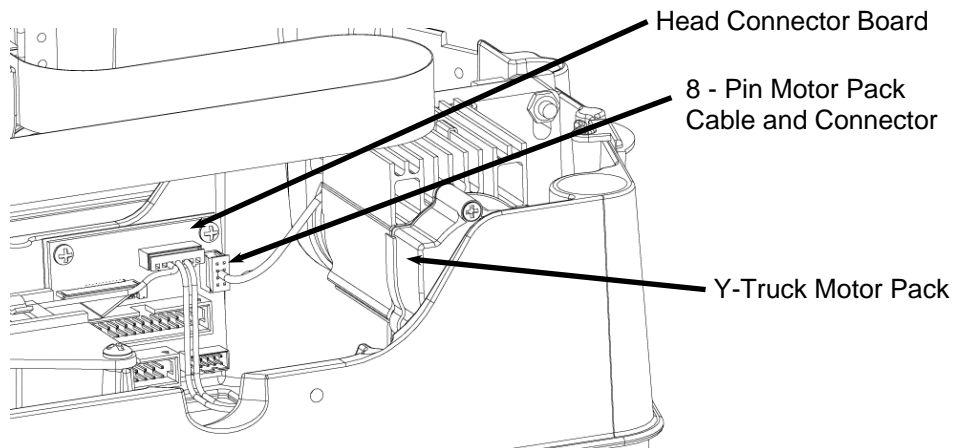
FIGURE 9: THE HEAD CONNECTOR BOARD
